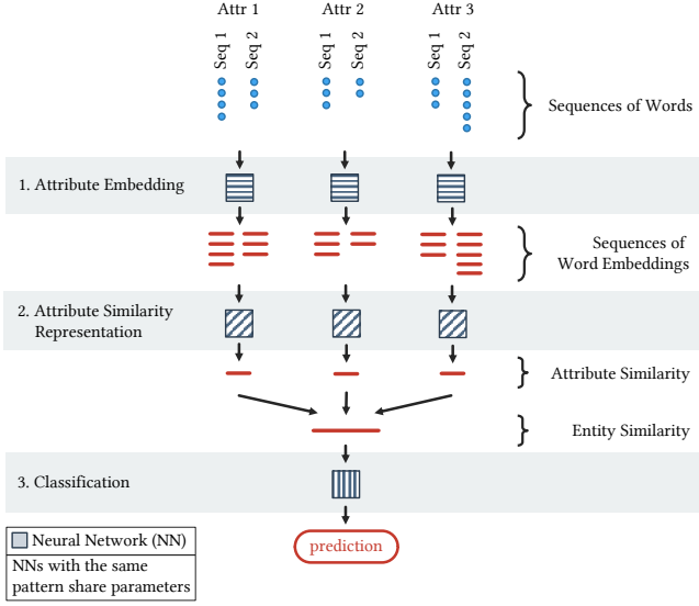
Figure 2: Our architecture template for DL solutions for EM. embedding or learn one from scratch), (2) the kind of network used to summarize the input, i.e., learn a vector representation of the input sequence pair (e.g., use an RNN or an attention-only mechanism or a combination of the two), and (3) the method used to compare the two input sequences (e.g., a neural network).
