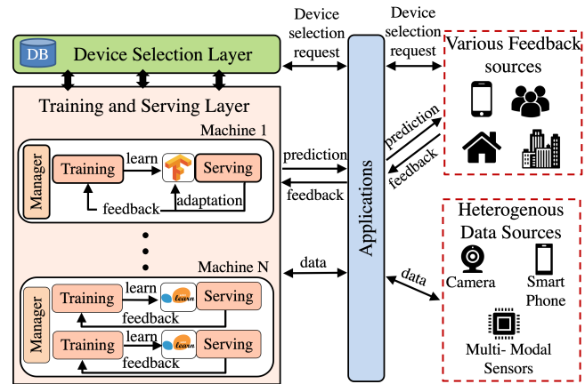
Figure 1: Overall System Architecture of MLIoT
