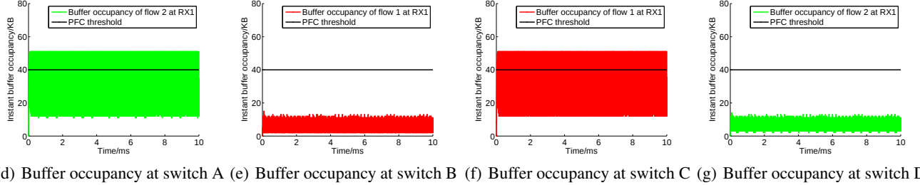
Figure 3: There is no deadlock even though two flows create cyclic buffer dependency among four switches.
